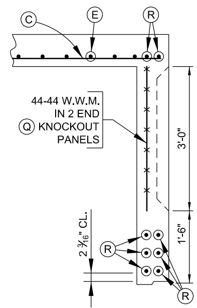
SECTION 2-2
